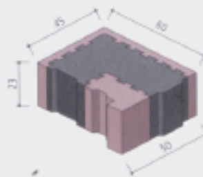
Eckstein 2
